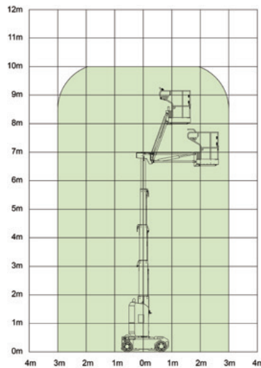
Range of motion ZMP08J
