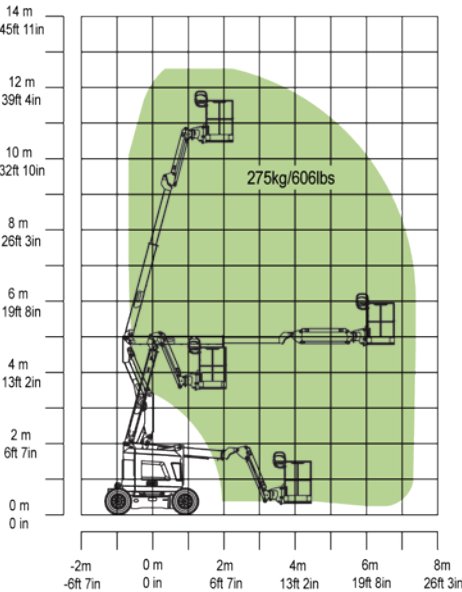
Range of Jib Swing Motion ZA10J
